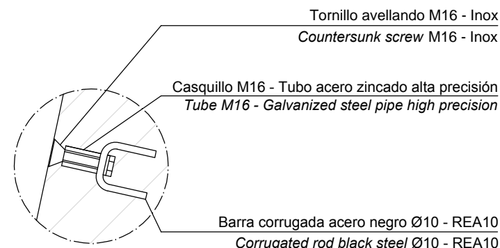
DETALLE / DETAIL
